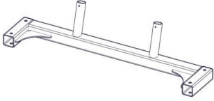
Rear Frame
